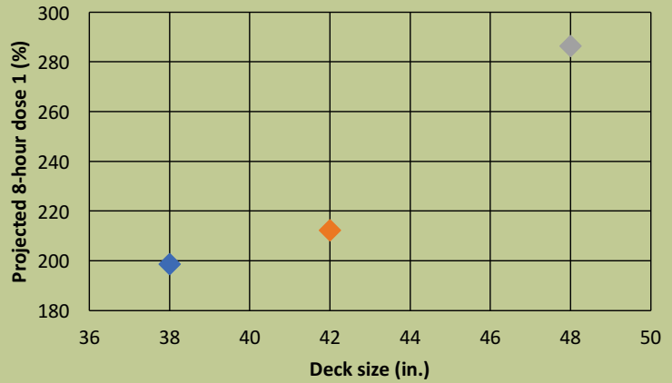
FIGURE 1 Effects of Deck Size on Noise Dose
